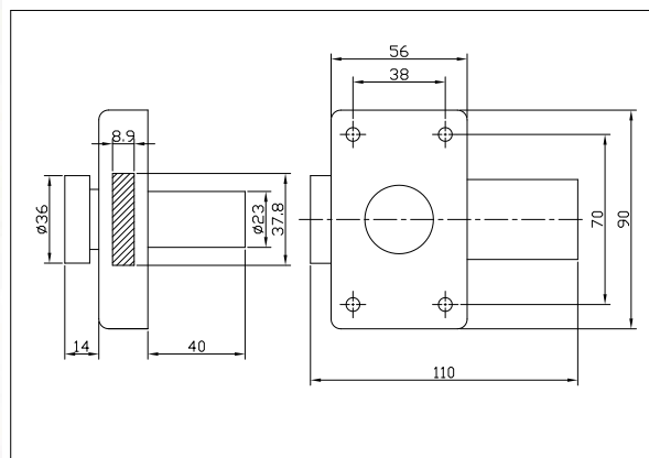
DL2673 Cellar Door Lock Cylinder Length: 40mm / 45mm / 50mm / 60mm
