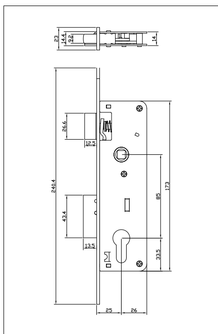
Backset 25 x c.c. 85 mm
