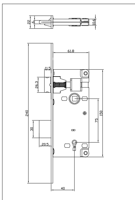
Backset 40 x c.c. 75 mm
