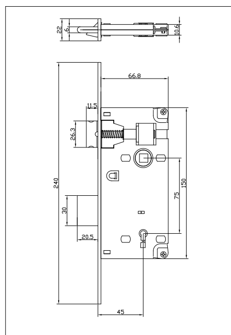
Backset 45 x c.c. 75 mm
