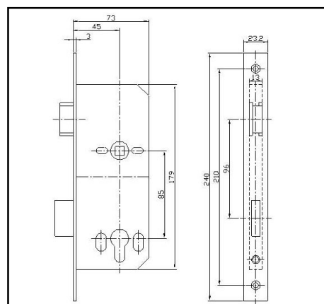
Backset 45 x c.c. 85 mm
