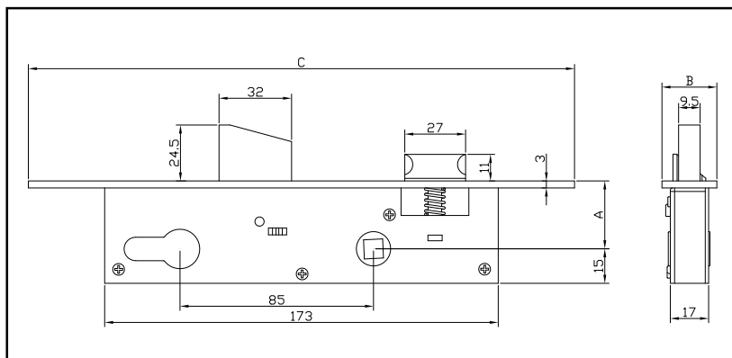
Centre 85mm, Backset 25mm / 30mm / 35mm
