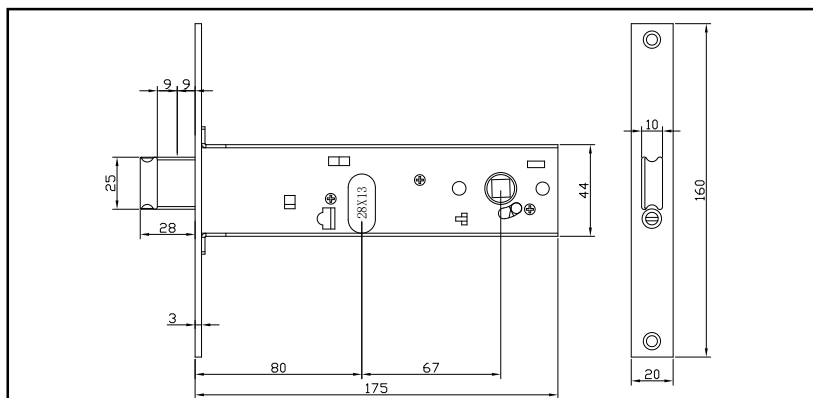
Backset 80 x c.c 67mm
