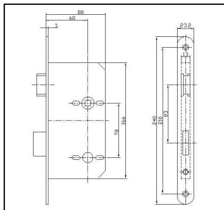
Backset 60 x c.c. 78 mm
