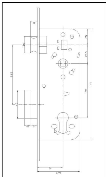
Backset 40 x c.c. 85 mm
