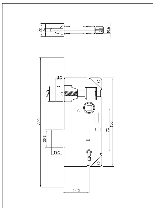
Backset 44.5 x c.c. 75 mm
