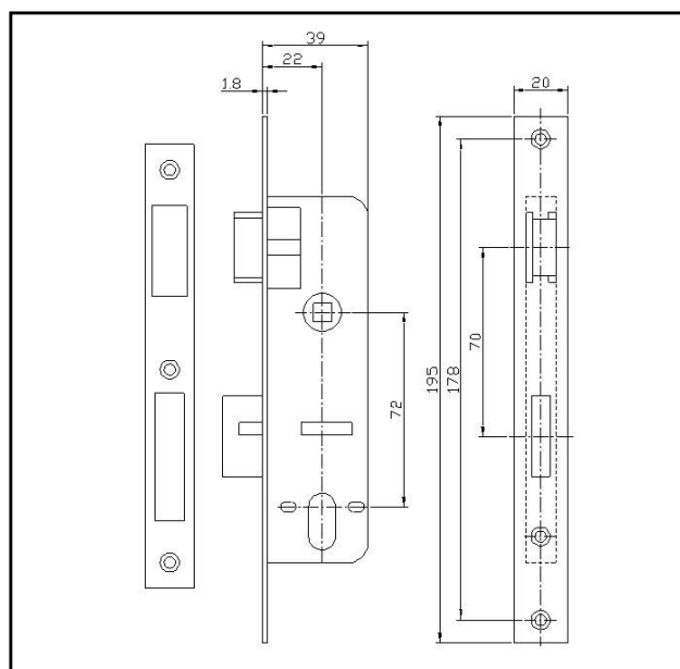
Backset 22 x c.c 72mm
