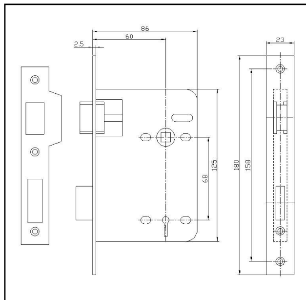
Backset 60 x c.c 68mm
