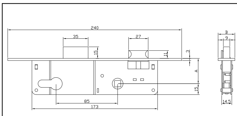
Centre 85mm, Backset 20mm / 25mm / 30mm / 35mm
